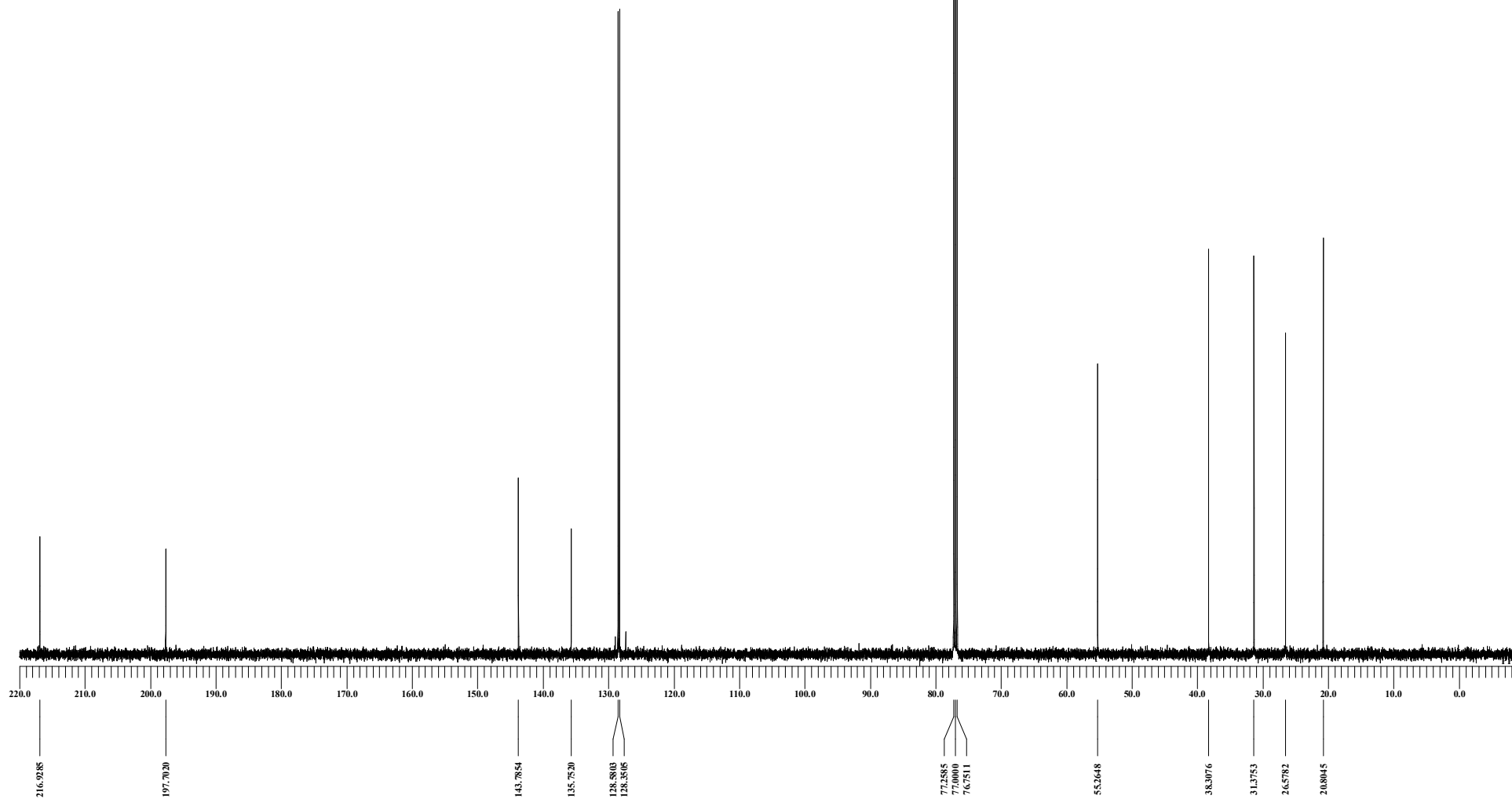
2-(4-acetylphenyl)cyclopentan-1-one (4) 13 C NMR (100 MHz, CDCl 3 )
