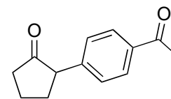
2-(4-acetylphenyl)cyclopentan-1-one (4) 13 C NMR (100 MHz, CDCl 3 )
